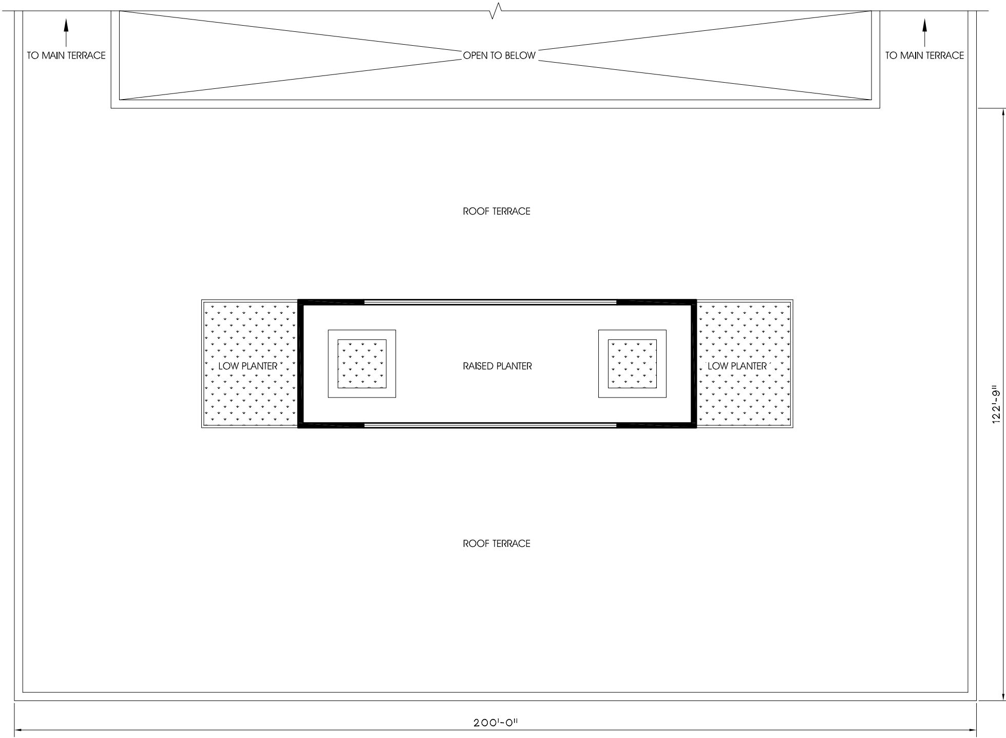
BUILDING "B" TERRACE PLAN
